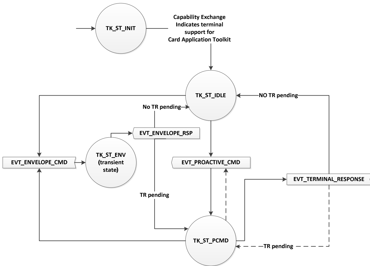
Figure 10.10: State transitions
